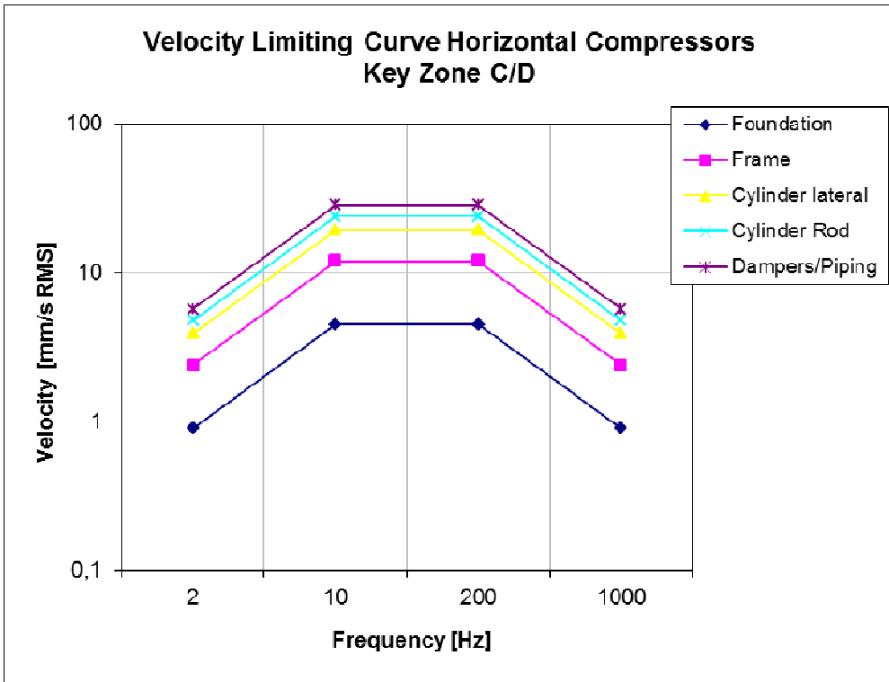
Figure 4.5.-Vibration velocity limiting curve for a horizontal compressor for key zone C/D.
