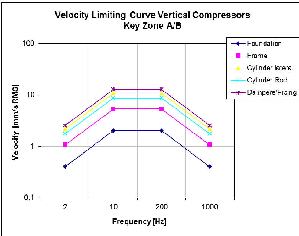
Figure 4.2. Vibration velocity limiting curve for a vertical compressor for key zone A/B.
