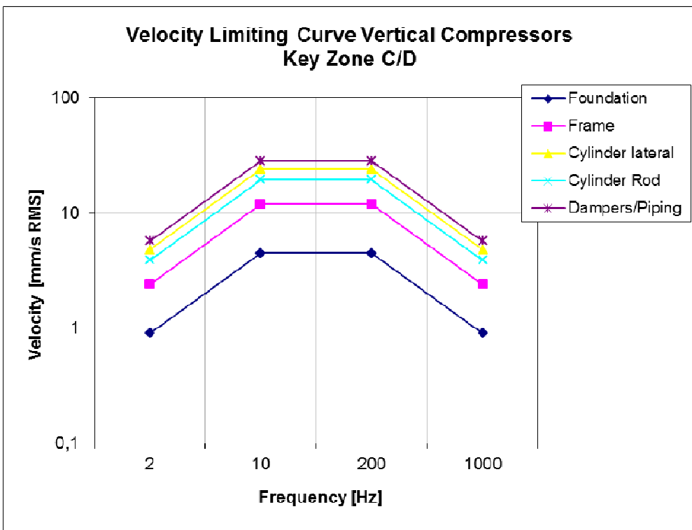
Figure 4.6.-Vibration velocity limiting curve for a vertical compressor for key zone C/D.
